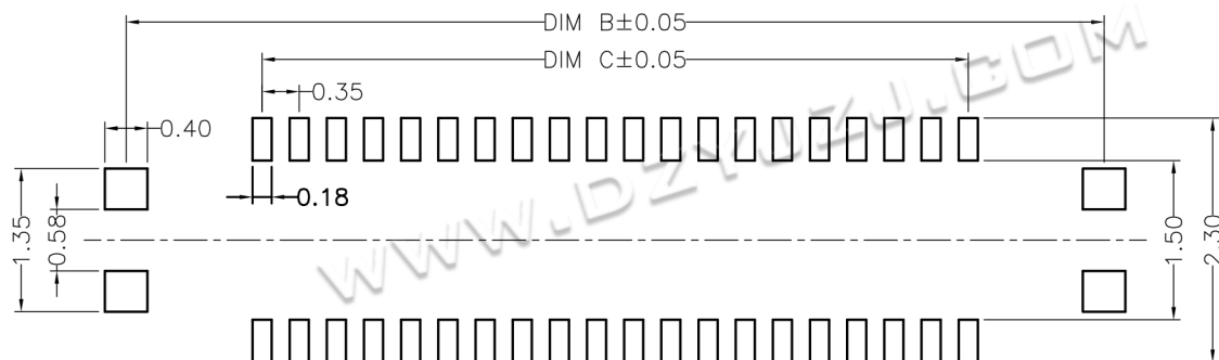
RECOMMENDED PCB LAYOUT CONNECTOR SIDE
